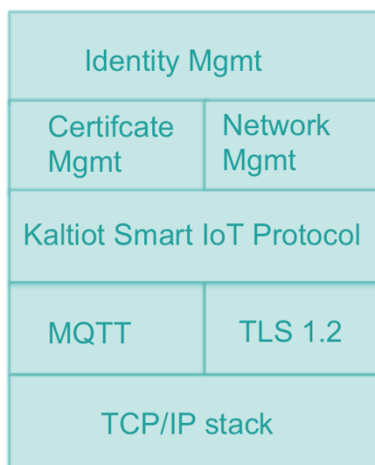
Figure: Client Stack (layered diagram)
